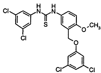
Compound # 45
